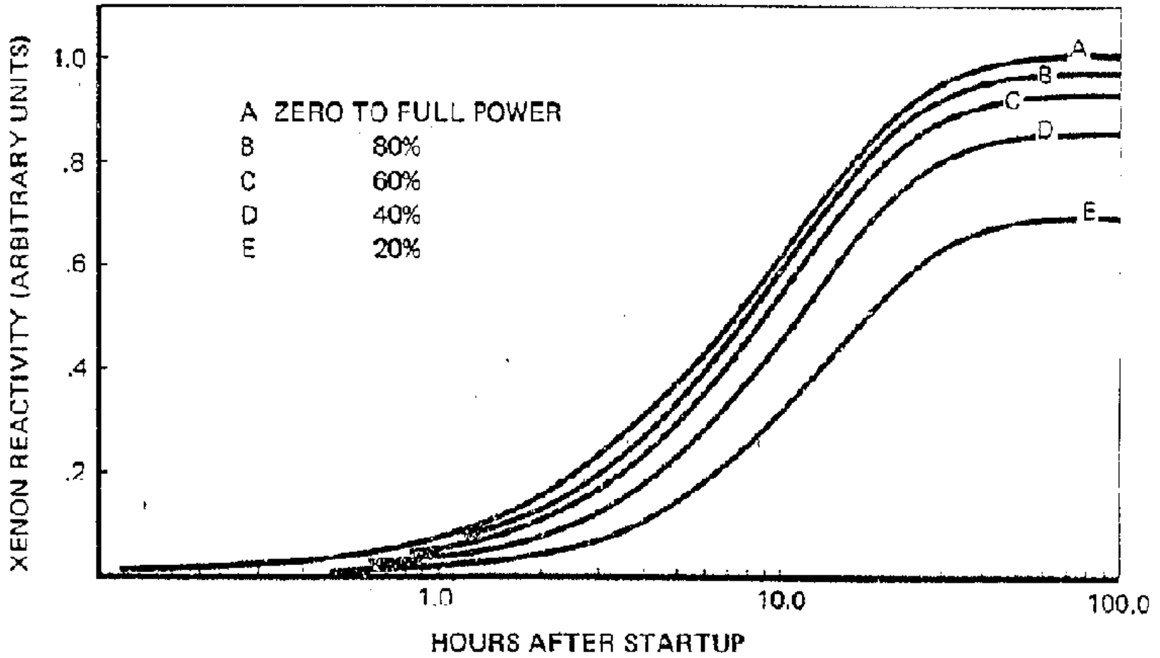
Figure 8.2 Xenon Reactivity After a Startup
