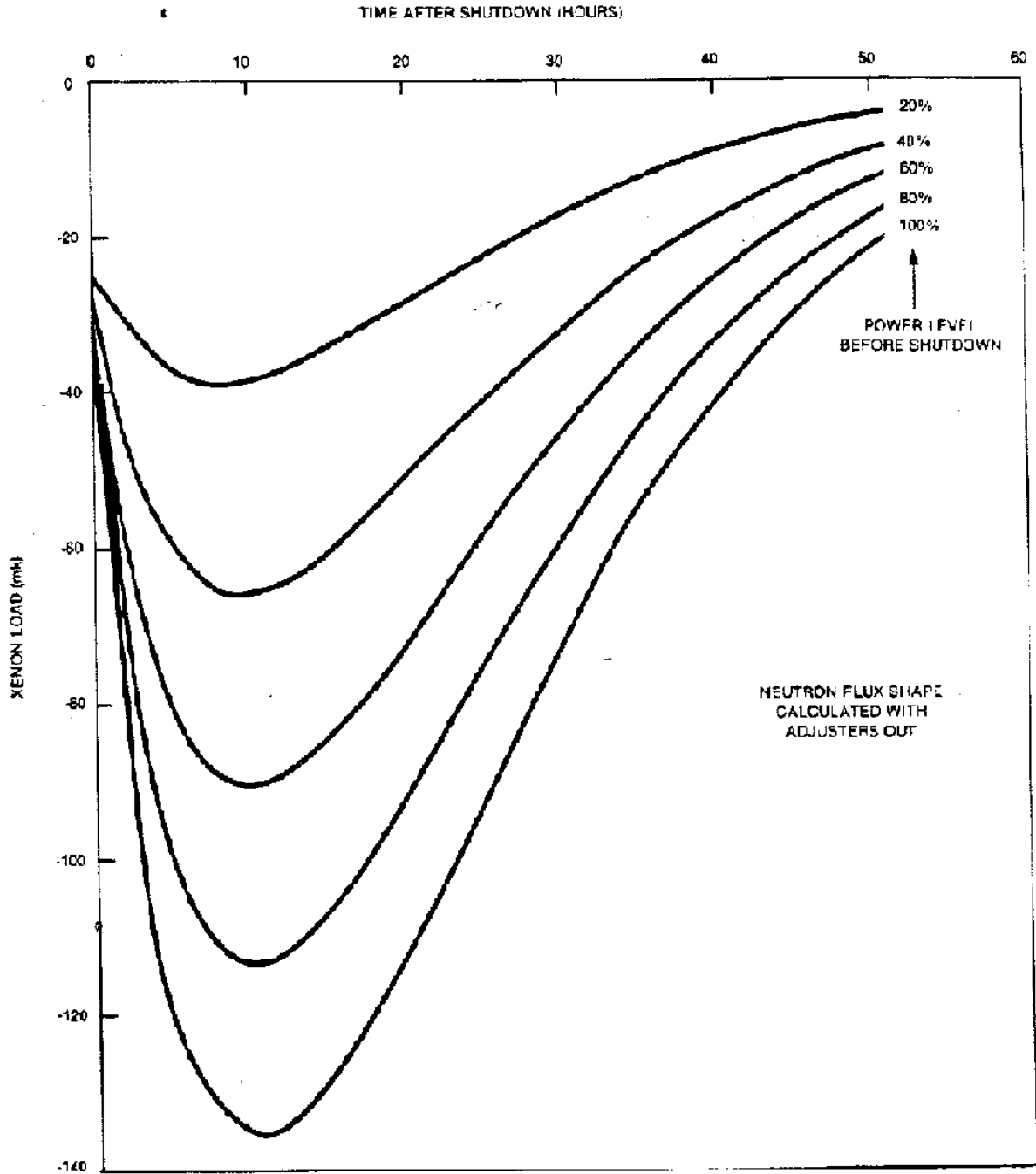
Figure 8.4 Xenon Transient Following Reactor Shutdown
